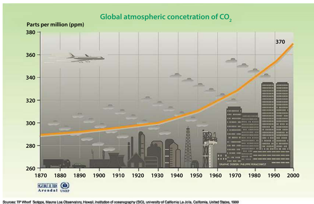
FIGURE 1: Global atmospheric concentration of CO 2
